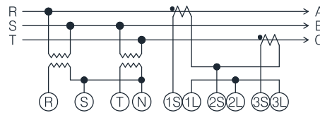
- 3P4W Connection -
