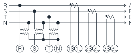
- 3P4W Connection -
