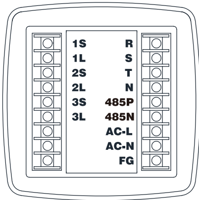
- Terminal Arrange -
